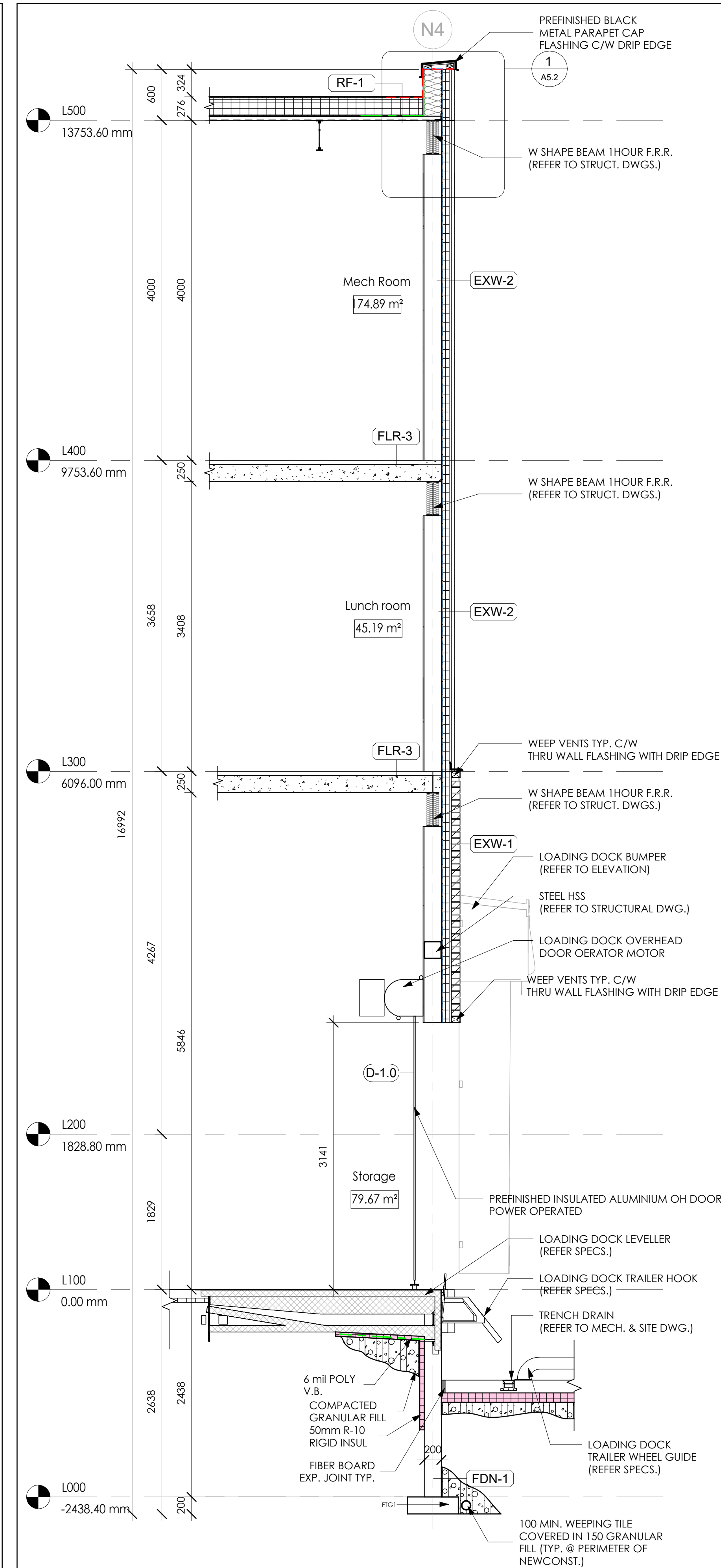
3 LOADING DOCK SECTION 1 : 35
