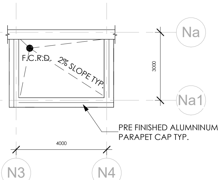
4 MAIN VEST. ROOF PLAN 1 : 100
