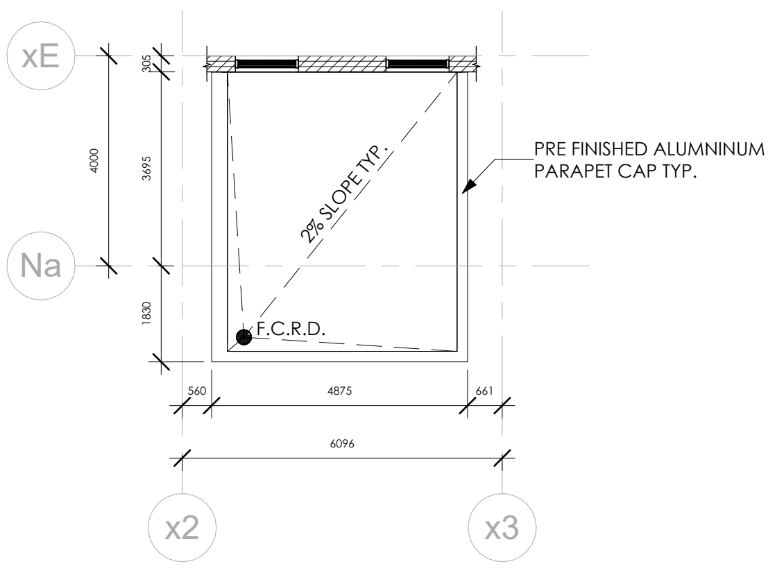
3 EXST.BLDG. CANOPY ROOF PLAN 1 : 100
