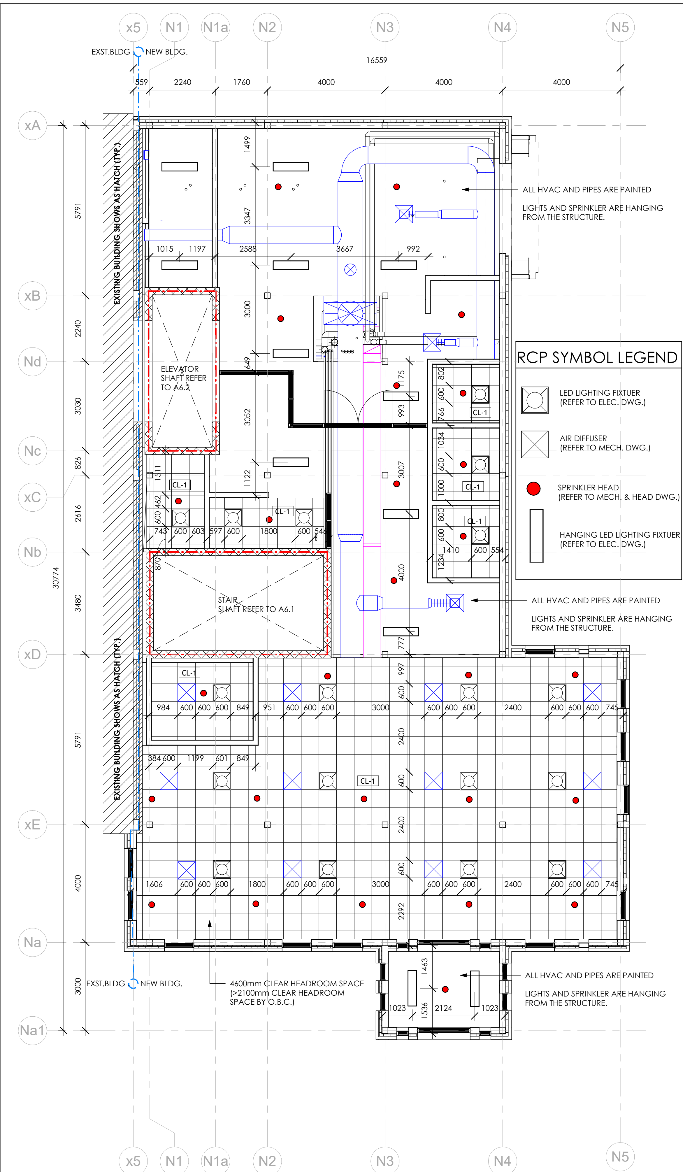
1 L100 ENLARGED R.C.P. MARKET PLAN 1:75
