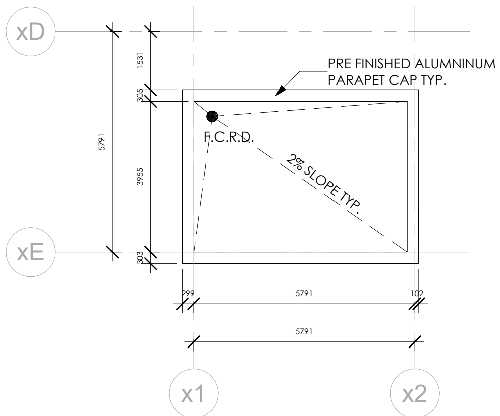
2 EXST.BLDG. STAIR ROOF PLAN 1 : 100
