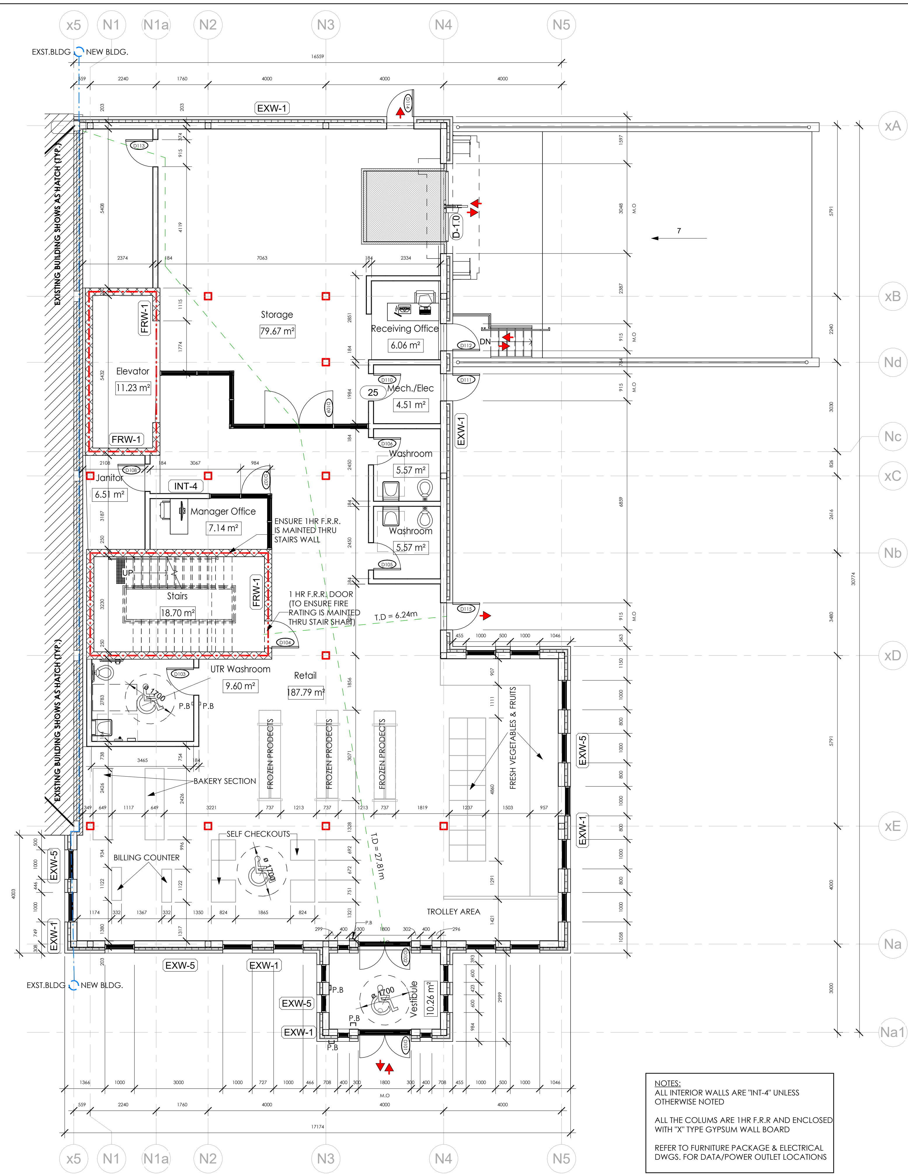
2 L100 ENLARGED MARKET PLAN 1:75
