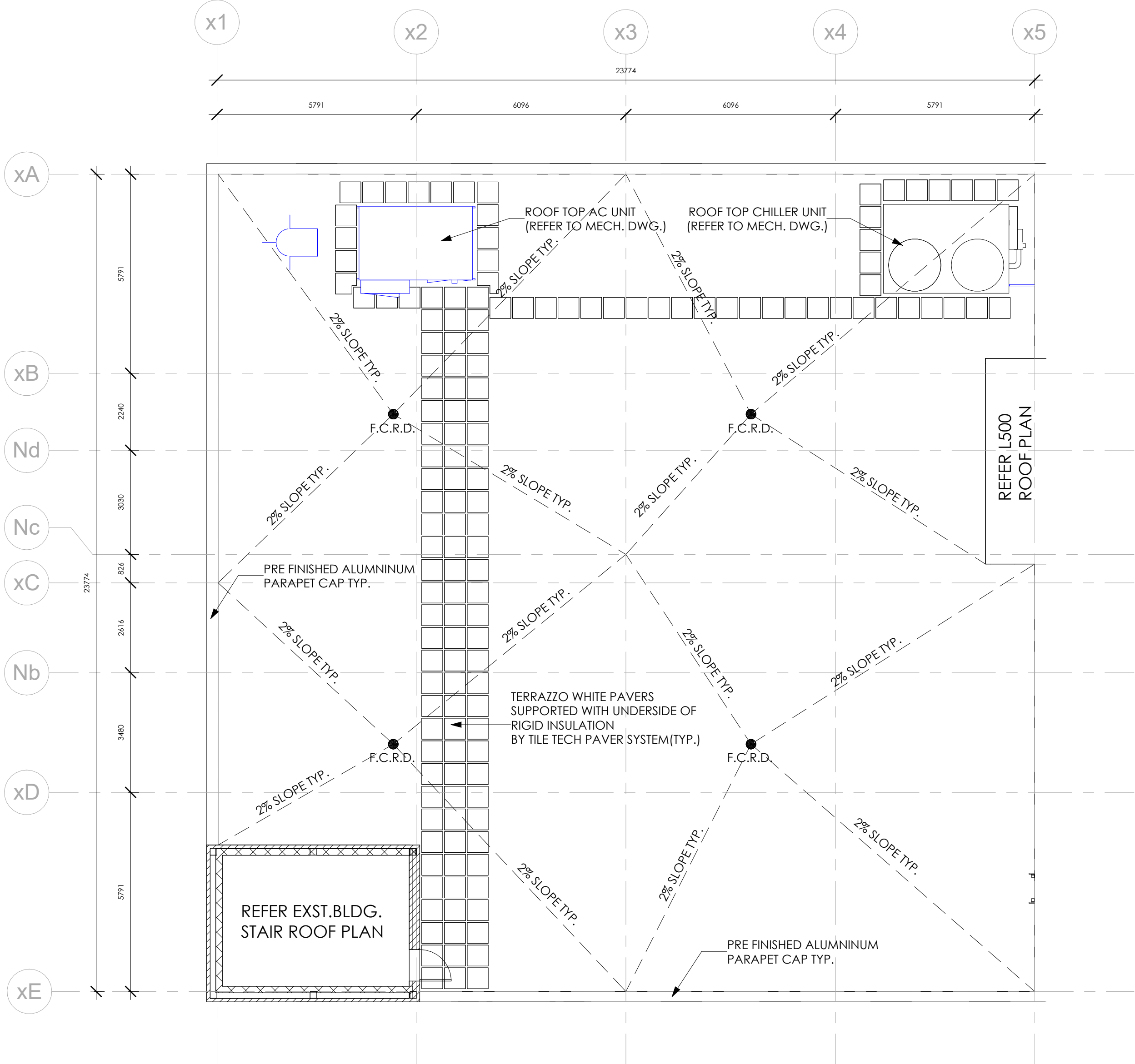
1 L400 ROOF PLAN 1 : 100
