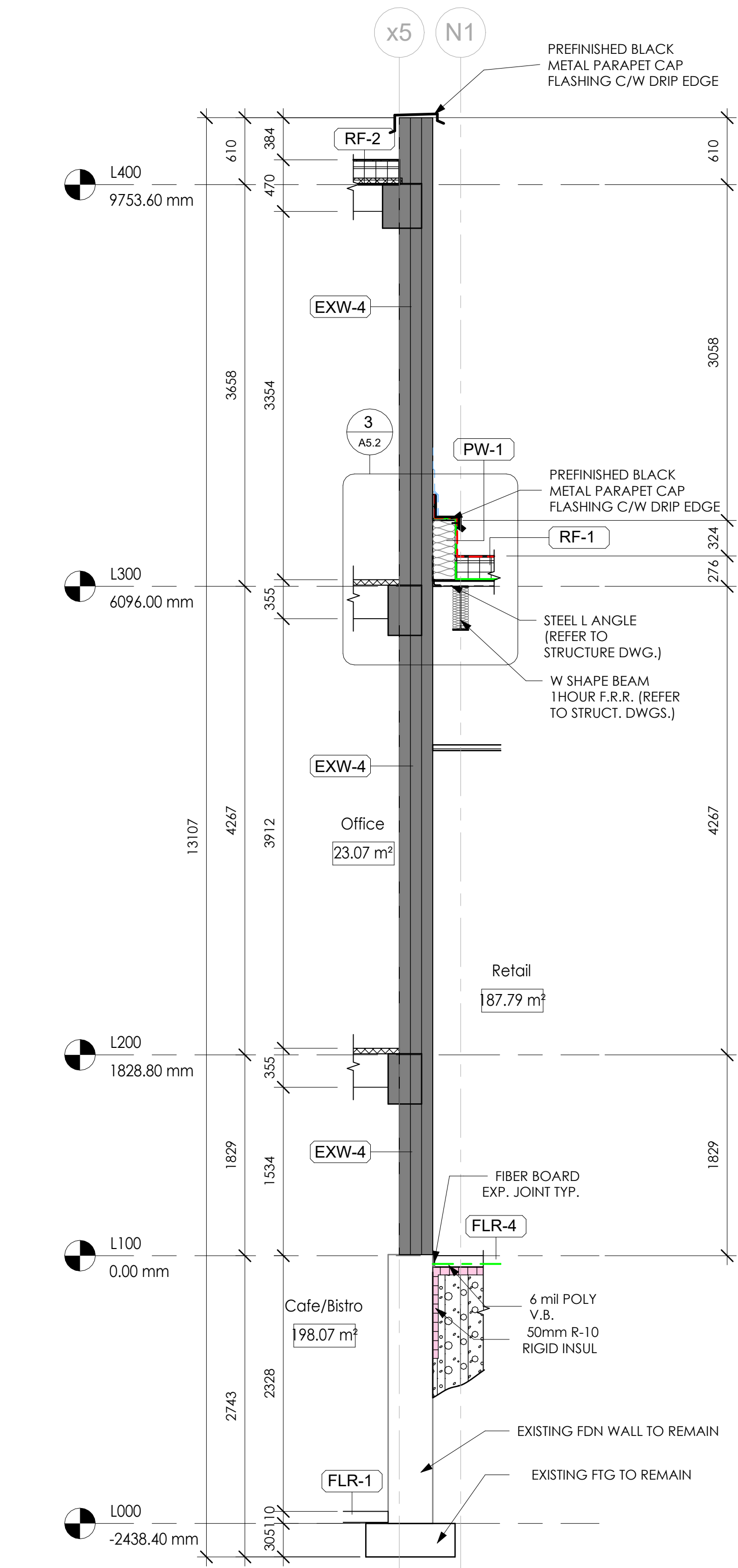
2 NEW TO EXISTING @ LOW ROOF 1 : 35
